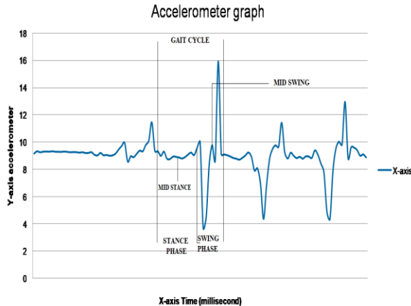
Fig.2 Graphical representation of gait cycle. From the graph it can be observed that stance phase occupies 60 percentage of gait cycle and swing phase occupies 40 percentage of gait-cycle.
