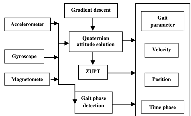
Fig.3 Overall system algorithm
