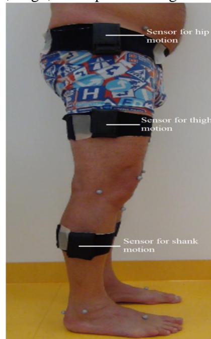
Fig.3 Placement of sensor on lower limbs
